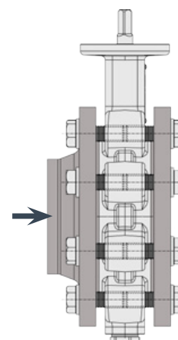
Type B installation with end piping
